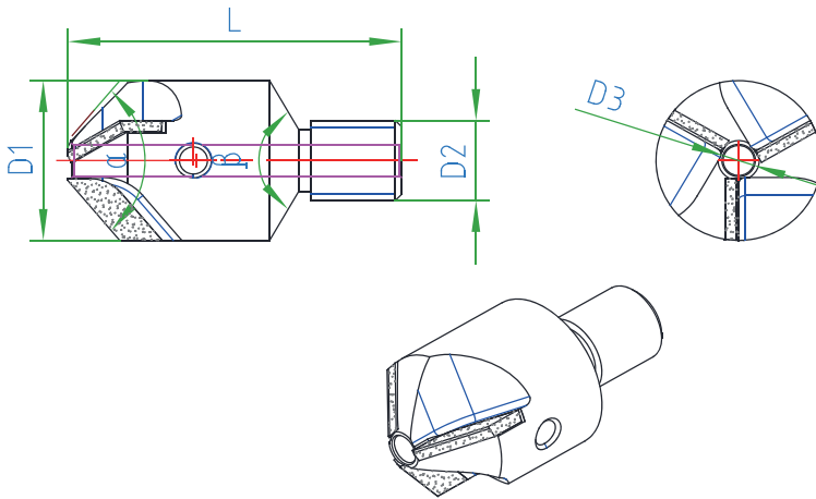
PCD socket drill with pin hole--Imperial
