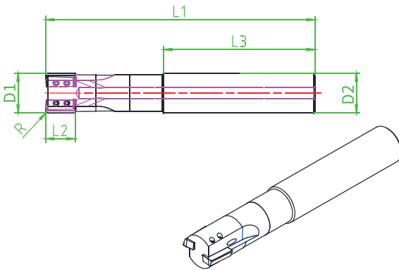
PCD quick change milling cutter-- Metric
