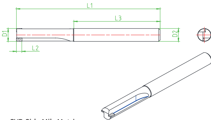
CVD Side Mill--Metric
