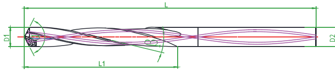
PCD twist drill-- Metric(with internal coolant)
