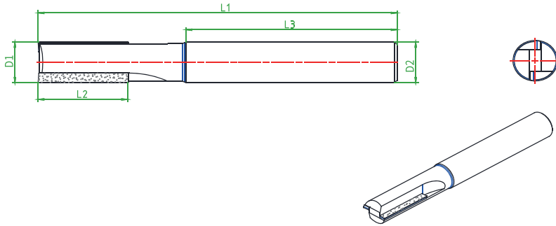
PCD milling cutter(not over center)--Imperial
